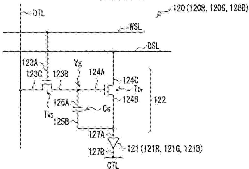
FIG. 16 PRIOR ART
